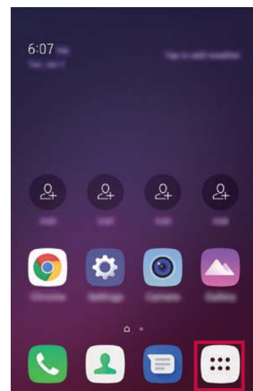
EasyHome
