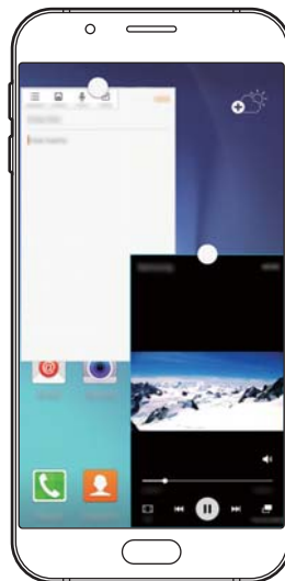
Pop-up view
