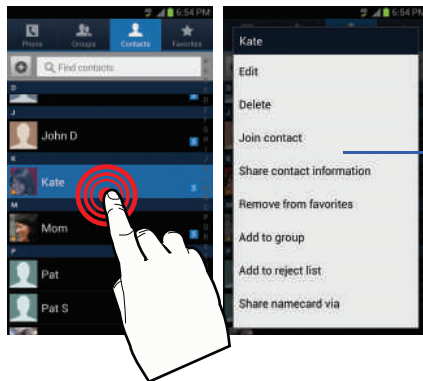
Context Menu
